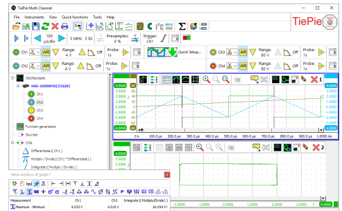
This measurement determines the area of an XY graph, using multiplying, integrating and differentiating I/O's. The area is indicated in the Value window: 16 V 2 .
