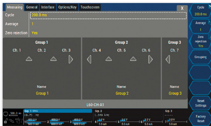
LMG600 with 7 power channels organised in 3 groups
